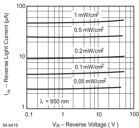
Fig. 5 Reverse Light Current vs. Reverse Voltage
