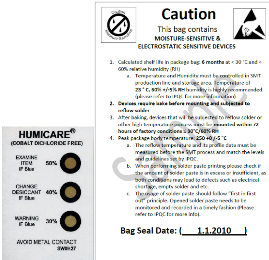
Figure 4: Example of moisture color coded card and caution label
