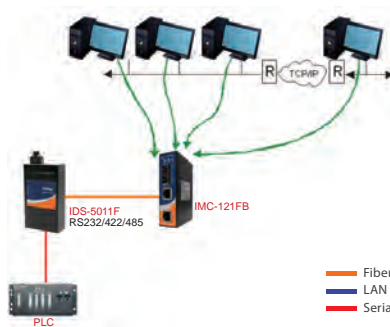
Multiple Host PCs
