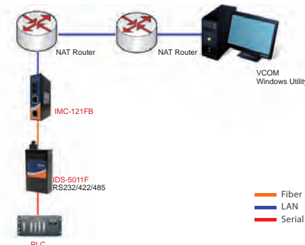
NAT Router Pass-Through
