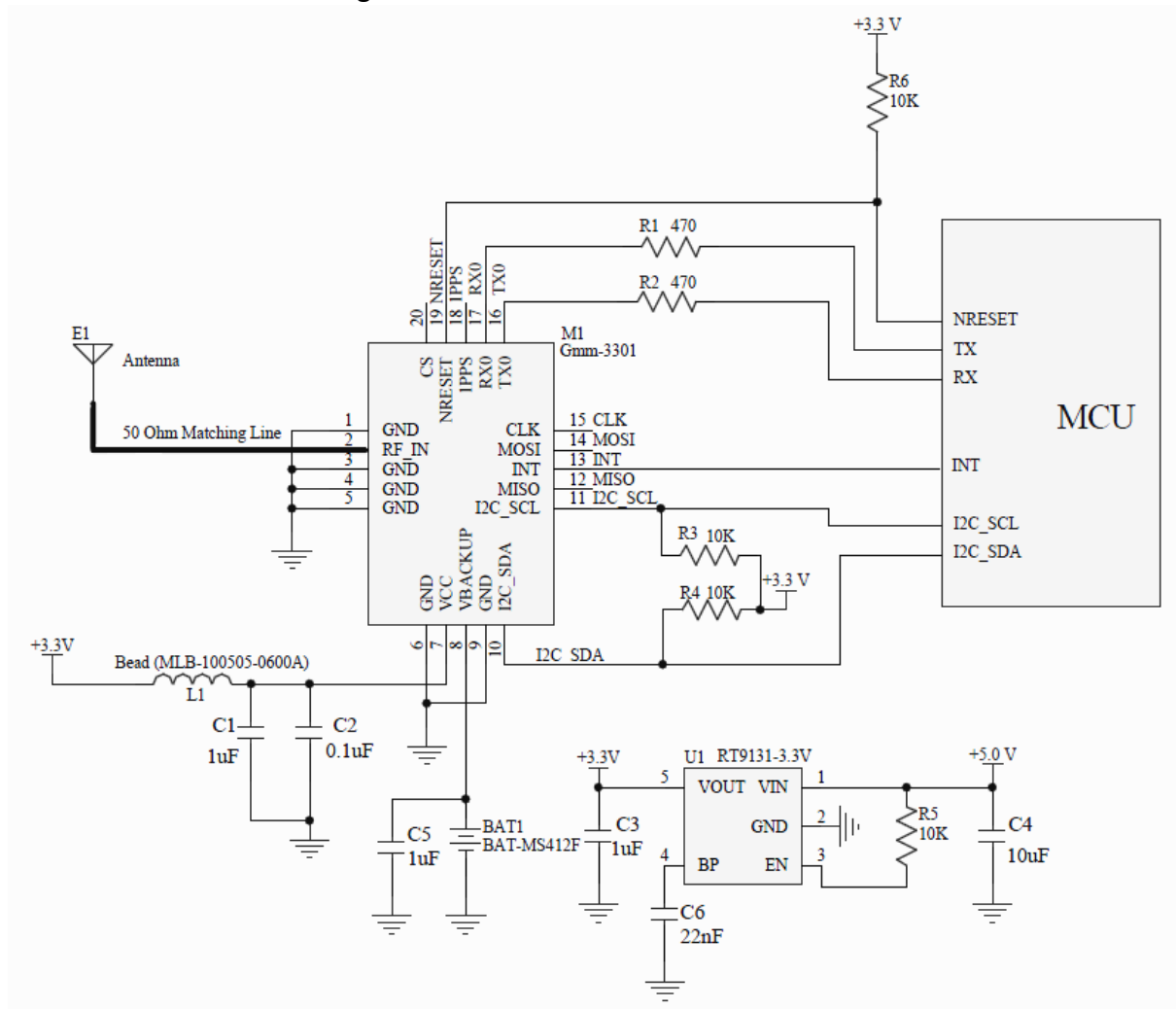
Fig. 4.2 UART+I2C application
