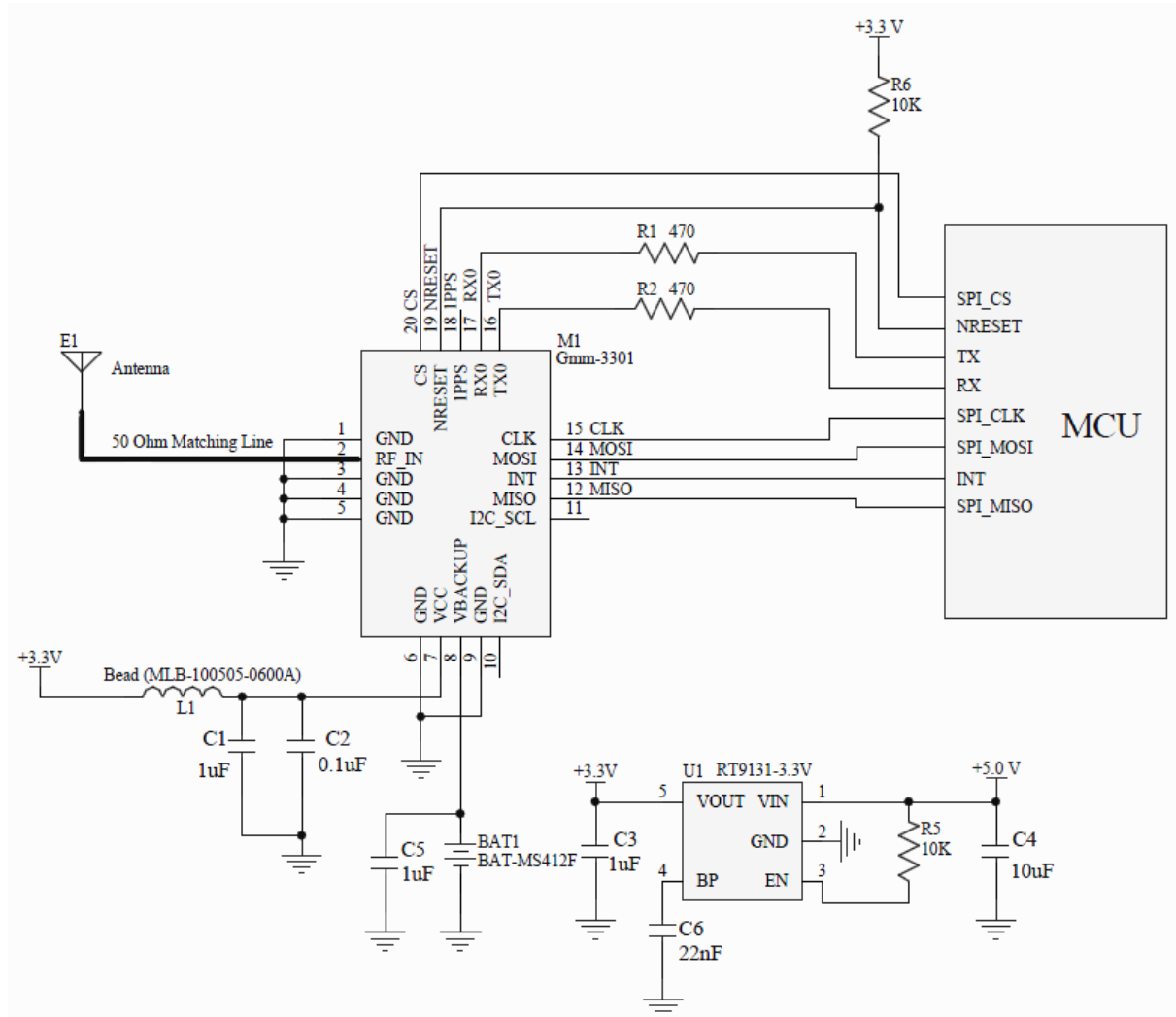
Fig. 4.3 UART+SPI application
